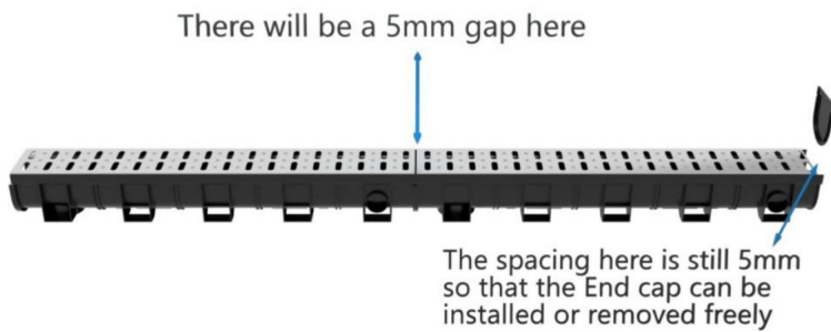
Pijpmontagemethode:
