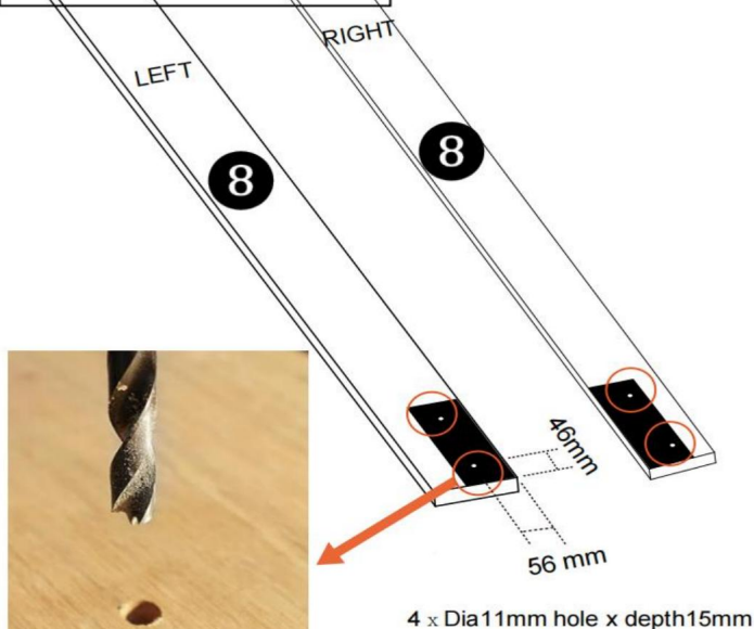
Use Dia11mm Wood Drill Bit
