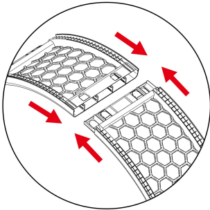
2. Runway frame assembly, assembled into a complete circle.
