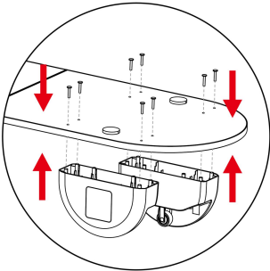
1. Fix the base with screws.
