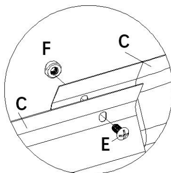
2.The connection of the straight plates.
