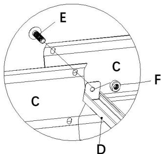
3.The connection of a connecting rod to a straight plate.
