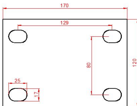
Parameters of mounting holes(mm)
