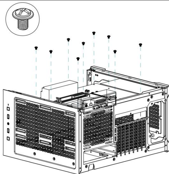
Installing the motherboard
