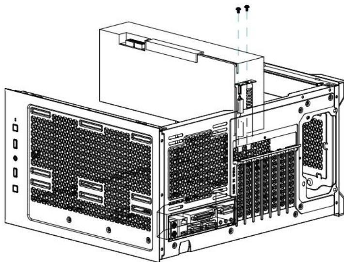
Installing a Graphics Card
