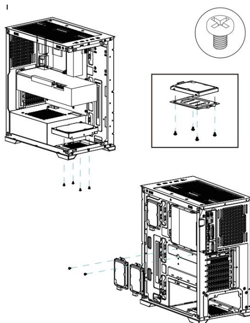
Installing SSD and HDD hard drives
