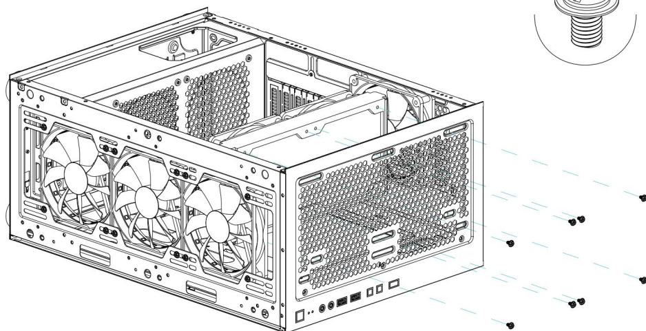
Installing the front /back panel fan
