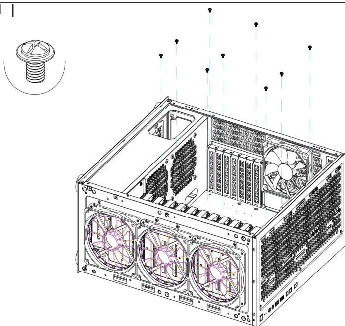
Installing the motherboard
