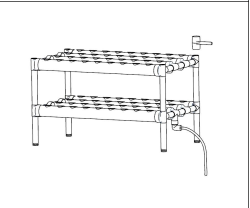
Figure 6: Connect the assembly of Figure 5 and the assembly of Figure 4 together. (Reinforce the four angles with a rubber hammer to adjust the level)
