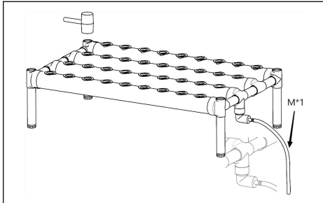
Figure 3: Connect the assembly of Figure 2 and the four foot tubes of Figure 1 together, and connect a 1m water outlet hose to the outlet tap. The hose should be cut to the appropriate length and kept straight to avoid affecting the flow rate. (Reinforce the four angles with a rubber hammer to adjust the level)
