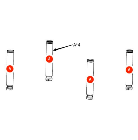
Figure 1: Prepare four 300mm foot tubes.
