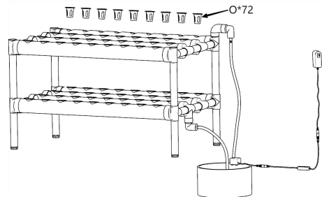
Figure 10: Put 72 planting baskets into the planting pipelines, and insert the adapter into the power supply. When the water pump works, it will form a water flow cycle. Finally, adjust the balance of the feet so that there is nutrient solution flowing through each pipe.
