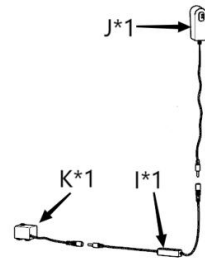
Figure 8: Connect an adapter, a controller, and a water pump together according to the diagram.
