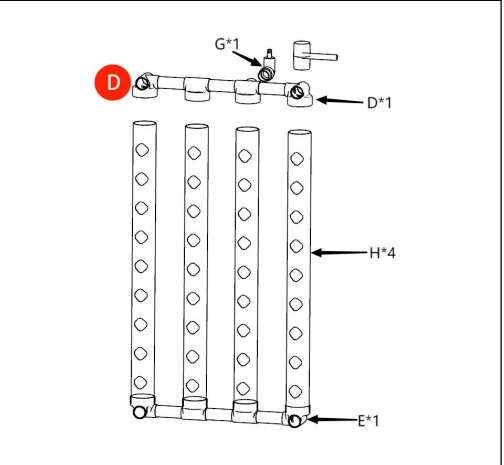
Figure 2: Connect a set of connector composite tubes, four planting pipelines, a set of water outlet composite pipes with letter D, and an outlet tap together according to the diagram, with the planting pipelines facing upwards. Reinforce them with a rubber hammer (strike each connection with the rubber hammer until they fit tightly)
