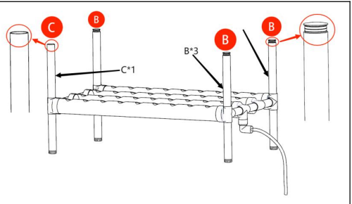
Figure 4: Connect three support tubes with letter B, one support tube with letter C, and the assembly of Figure 3 together according to the diagram. (Note that the support tube without a water plug should be placed in the bottom left corner)
