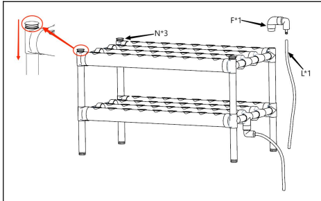
Figure 7: Connect three dust plugs, an inlet tap and a 1.5m hose together according to the diagram. The hose should be cut to the appropriate length and kept straight to avoid affecting the flow rate.
