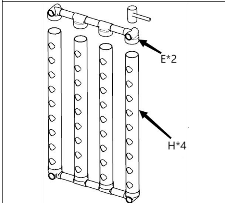
Figure 5: Connect two sets of connector composite tubes and four planting pipelines together according to the diagram, with the planting pipelines facing upwards. Reinforce them with a rubber hammer (strike each connection with the rubber hammer until they fit tightly)
