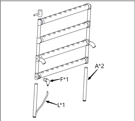
Figure 2: Connect two 400mm foot tubes, a 1m hose and an outlet tap with the assembly of Figure 1 according to the diagram. (Reinforce the two angles with a rubber hammer to adjust the level)
