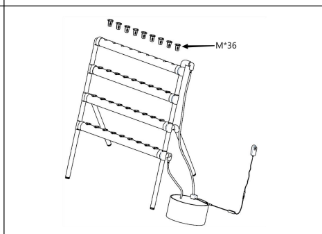
Figure 6: Put 36 planting baskets into the planting pipelines, and insert the adapter into the power supply. When the water pump works, it will form a water flow cycle. Finally, adjust the balance of the feet so that there is nutrient solution flowing through each pipe.
