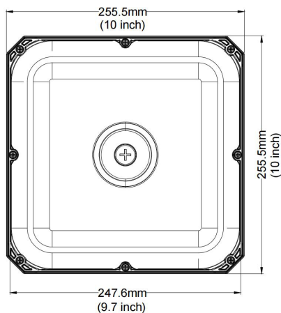
MODEL:GT-TPD4-80W
