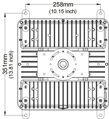
MODEL:GT-TPD-150W/GT-TPD4-150W
