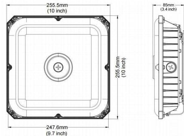
MODEL:GT-TPD4-80W
