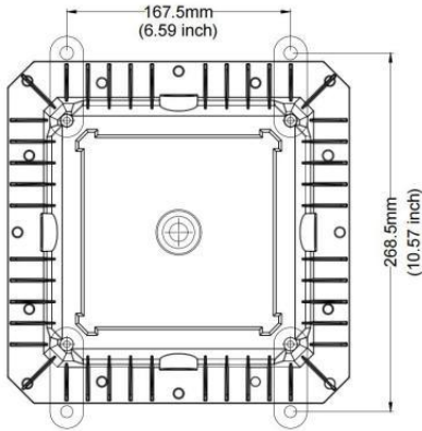
MODEL:GT-TPD4-80W
