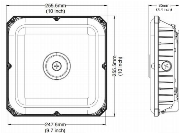
MODEL:GT-TPD4-80W
