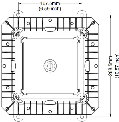
MODEL:GT-TPD4-80W
