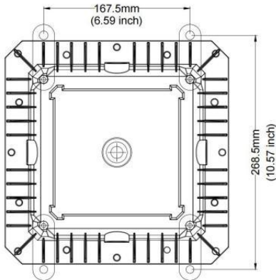
MODEL:GT-TPD4-80W
