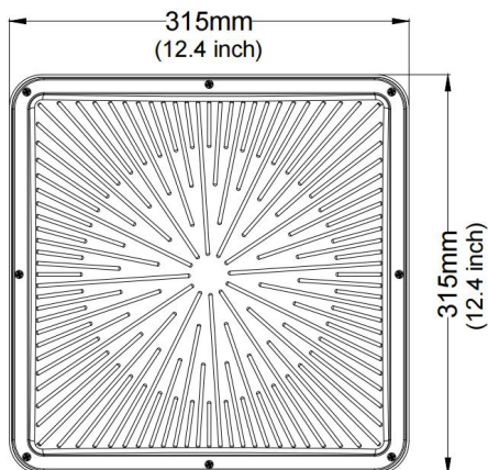
MODEL:GT-TPD4-80W
