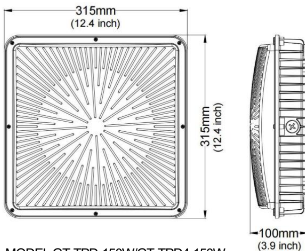
MODEL:GT-TPD-150W/GT-TPD4-150W
