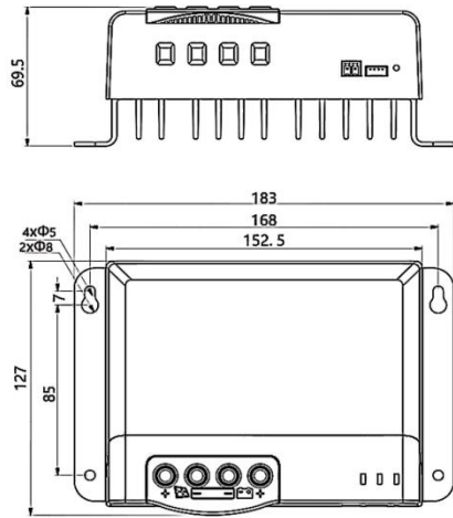
Model: MC2450N10-B; Outline dimensions: 183*127*69.5mm; Mounting dimensions: 168*85mm; Fixed holes dia: \Phi 5mm; Wire specifications: 20-6AWG.
